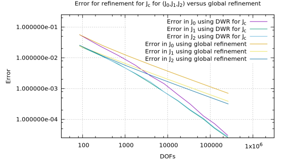
Figure 33: Example 4a: Error for Config. 3.
