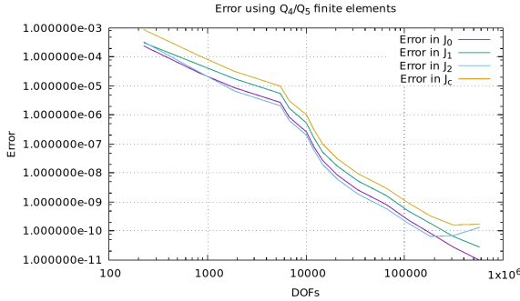
Figure 23: Example 3: Error using Q_4/Q_5 finite elements.
