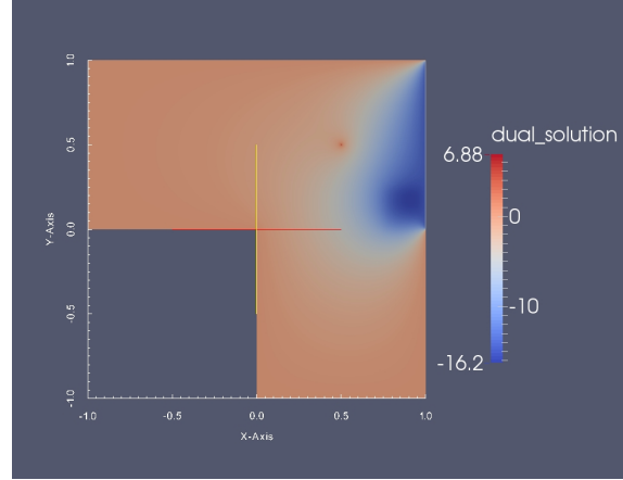
Figure 20: Example 2b: Dual solution after 7 refinement steps.
