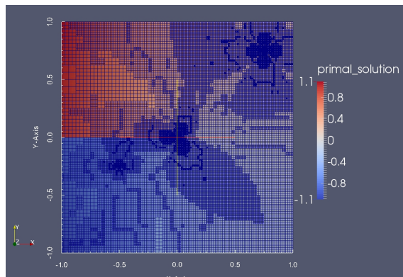
Figure 37: Example 4a: Mesh for Config. 2 after 7 refinement steps (49883 DOFs).
