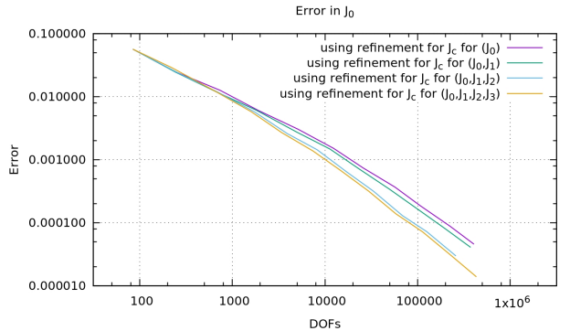
Figure 35: Example 4a: Error for J_0 for Configuration 1-4.
