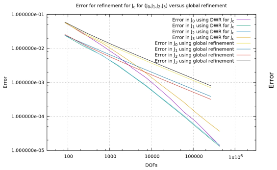
Figure 34: Example 4a: Error for Config. 4.
