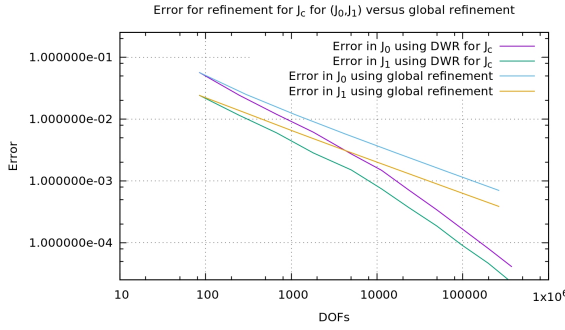
Figure 32: Example 4a: Error for Config. 2.
