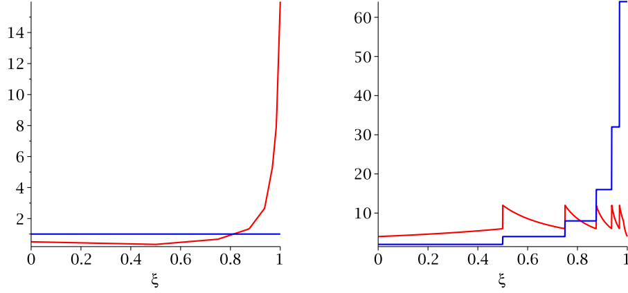
Figure 7: Compensation of a non-uniform knot vector by a suitable geometry mapping: The function \omega (left) and the term \frac{1}{h\epsilon\omega} (right) for the identity mapping (blue) and the mapping with equidistant control points (red).
